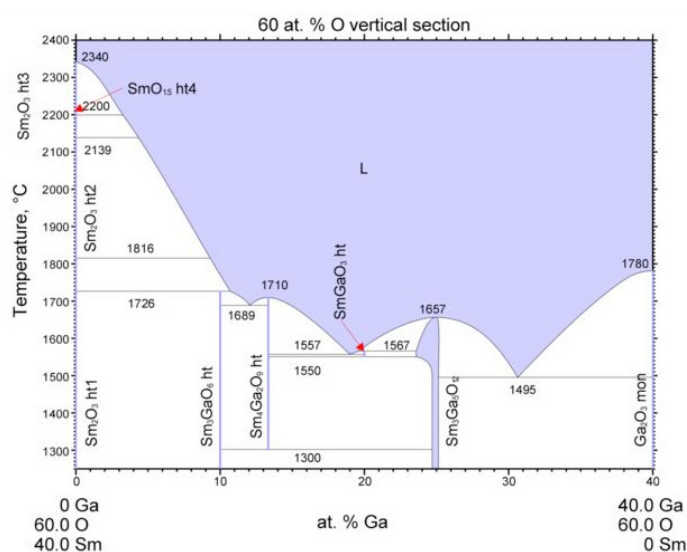
Fig. 1. The state diagram of the triple system Sm — Ga — O [3]
